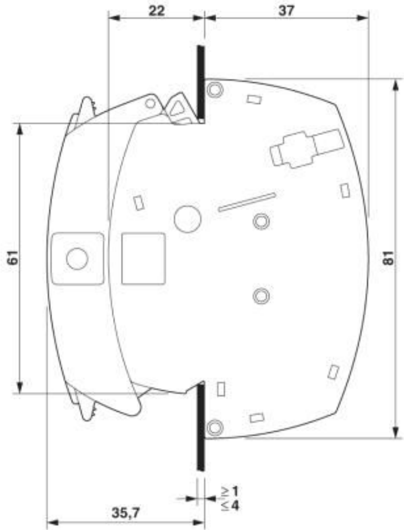
Dimensional drawing
