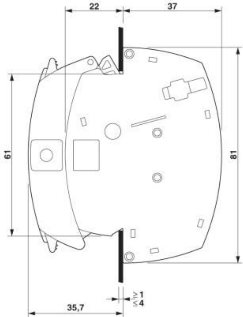
Dimensional drawing
