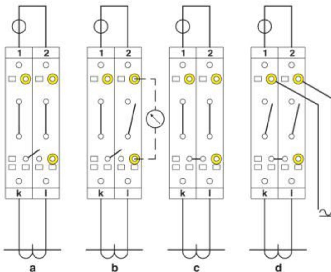
Connection diagram
