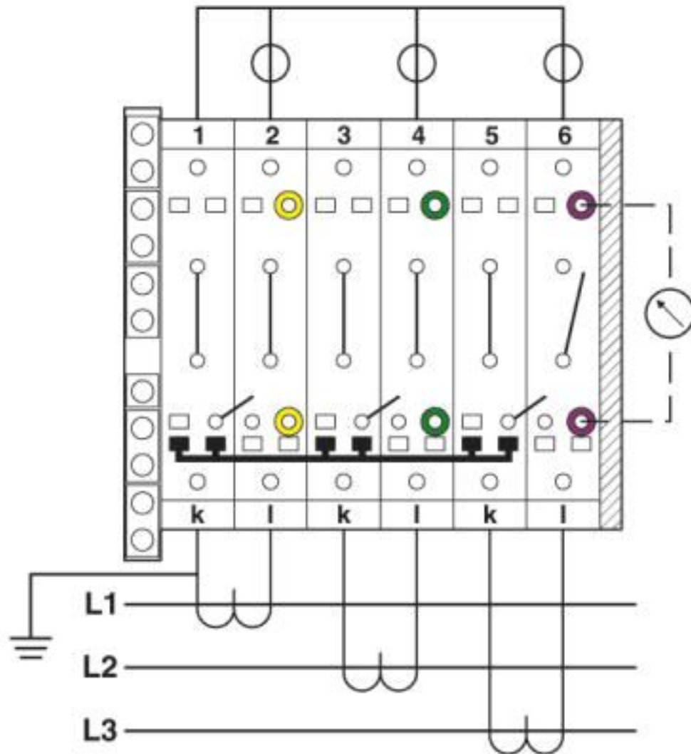
Connection diagram
