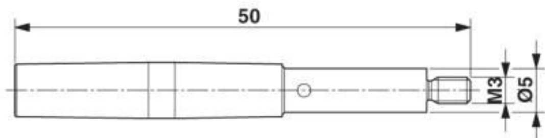
Dimensional drawing
