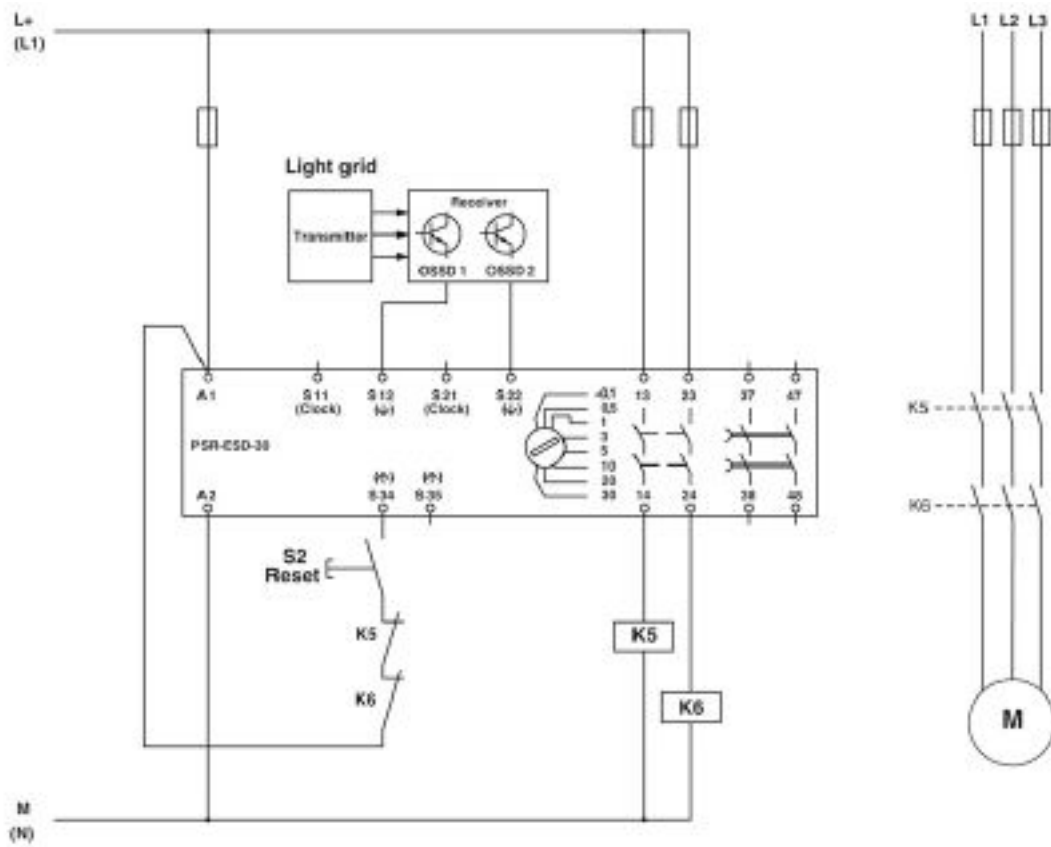
Circuit diagram
