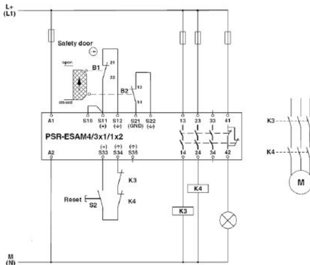
Circuit diagram
