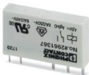
Plug-in miniature power relay, with power contact, 1 PDT, input voltage 4.5 V DC
