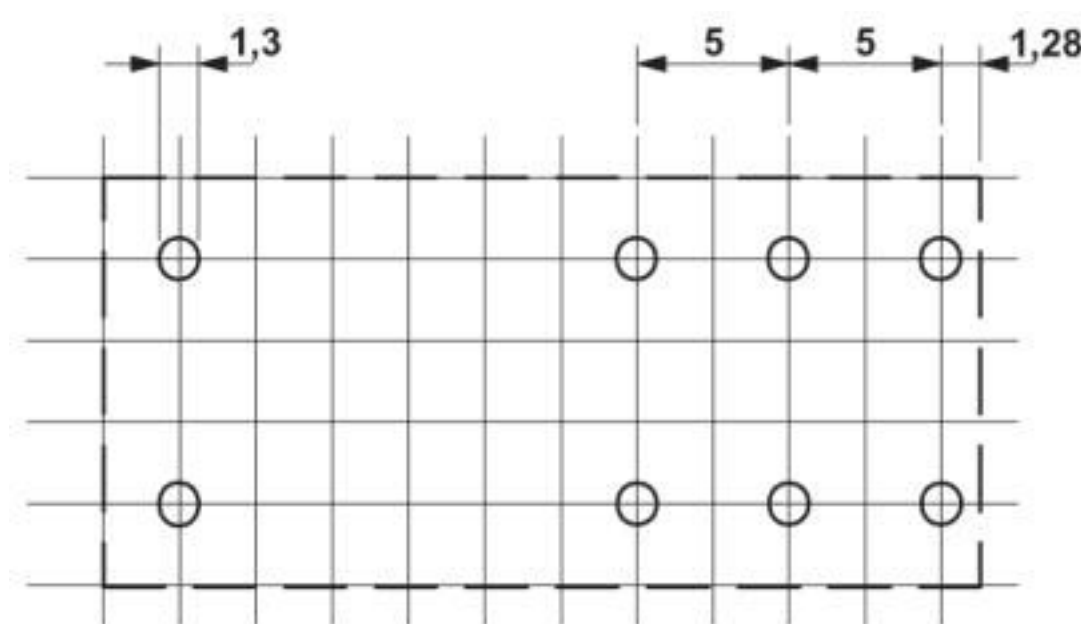
Drilling diagram
