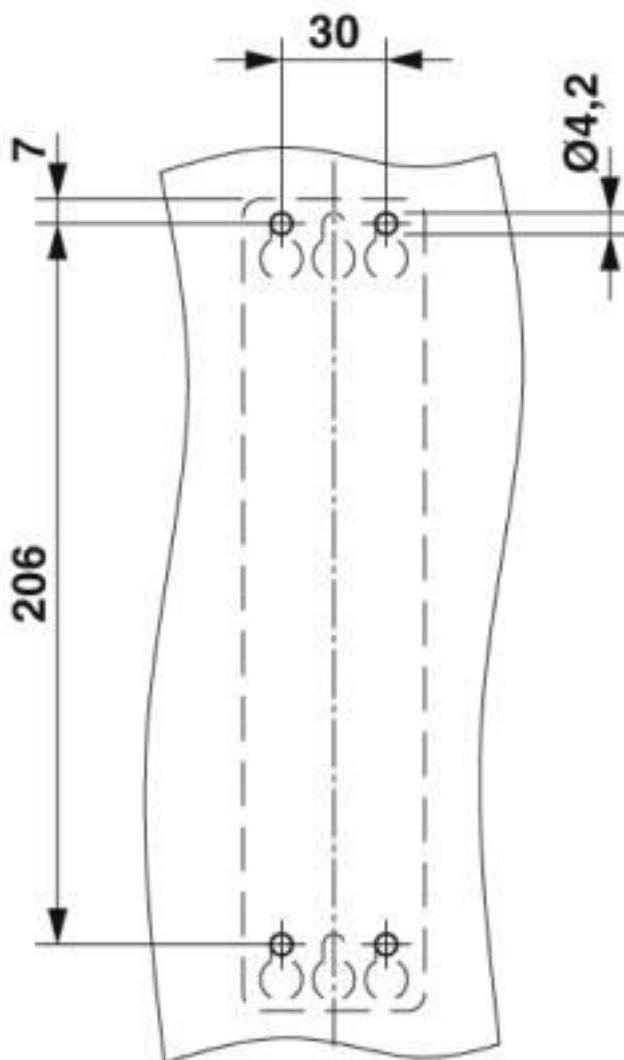
Drilling diagram
