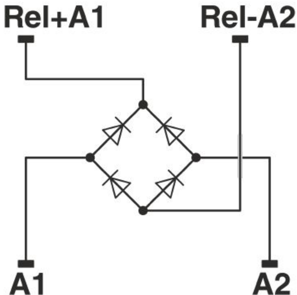
Circuit diagram
