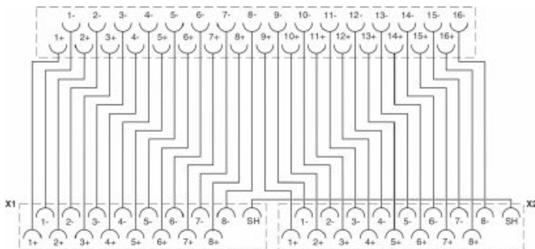
Circuit diagram
