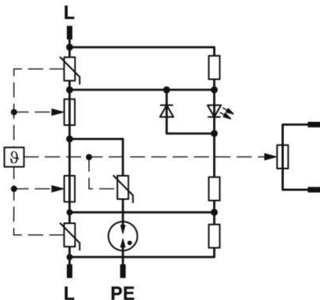
Circuit diagram
