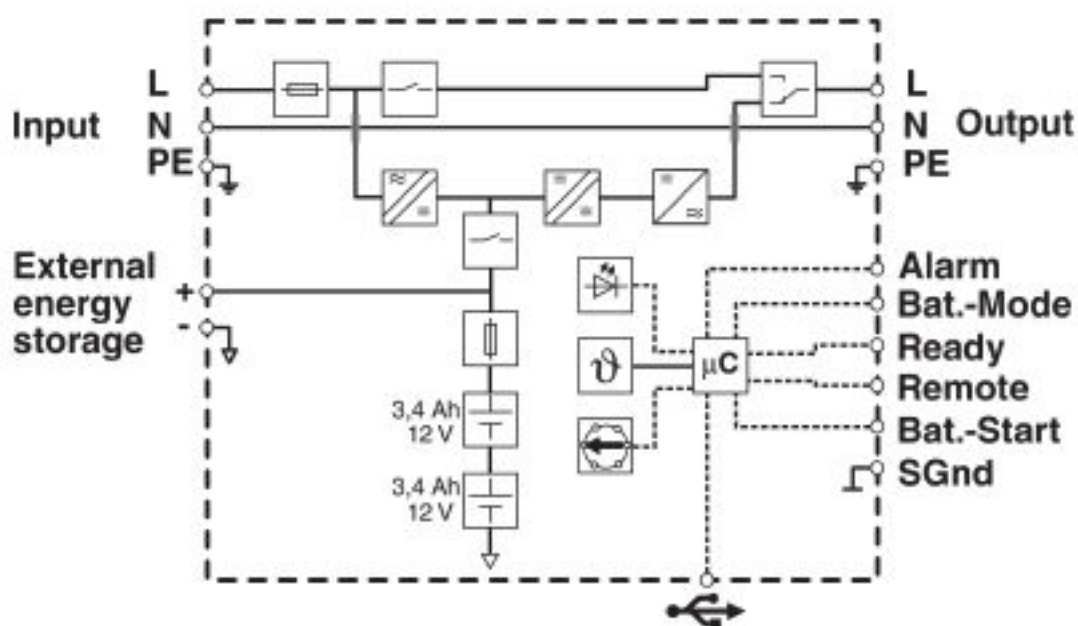
Block diagram
