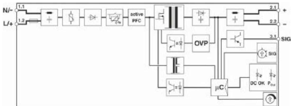
Block diagram
