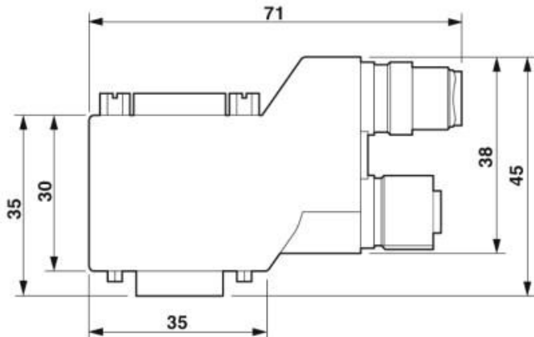
SUBCON-PLUS...90...M12 dimensional drawing, short 90° version
