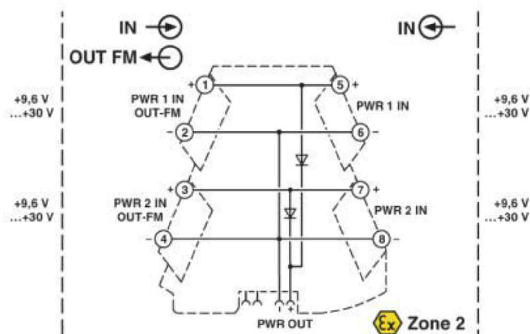
Block diagram
