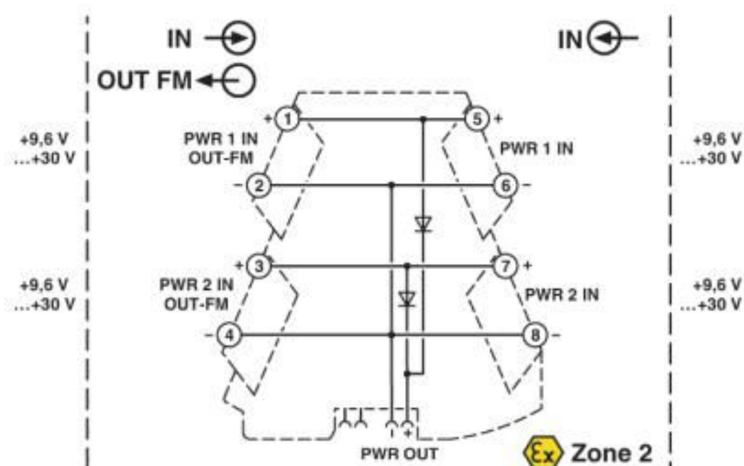
Block diagram
