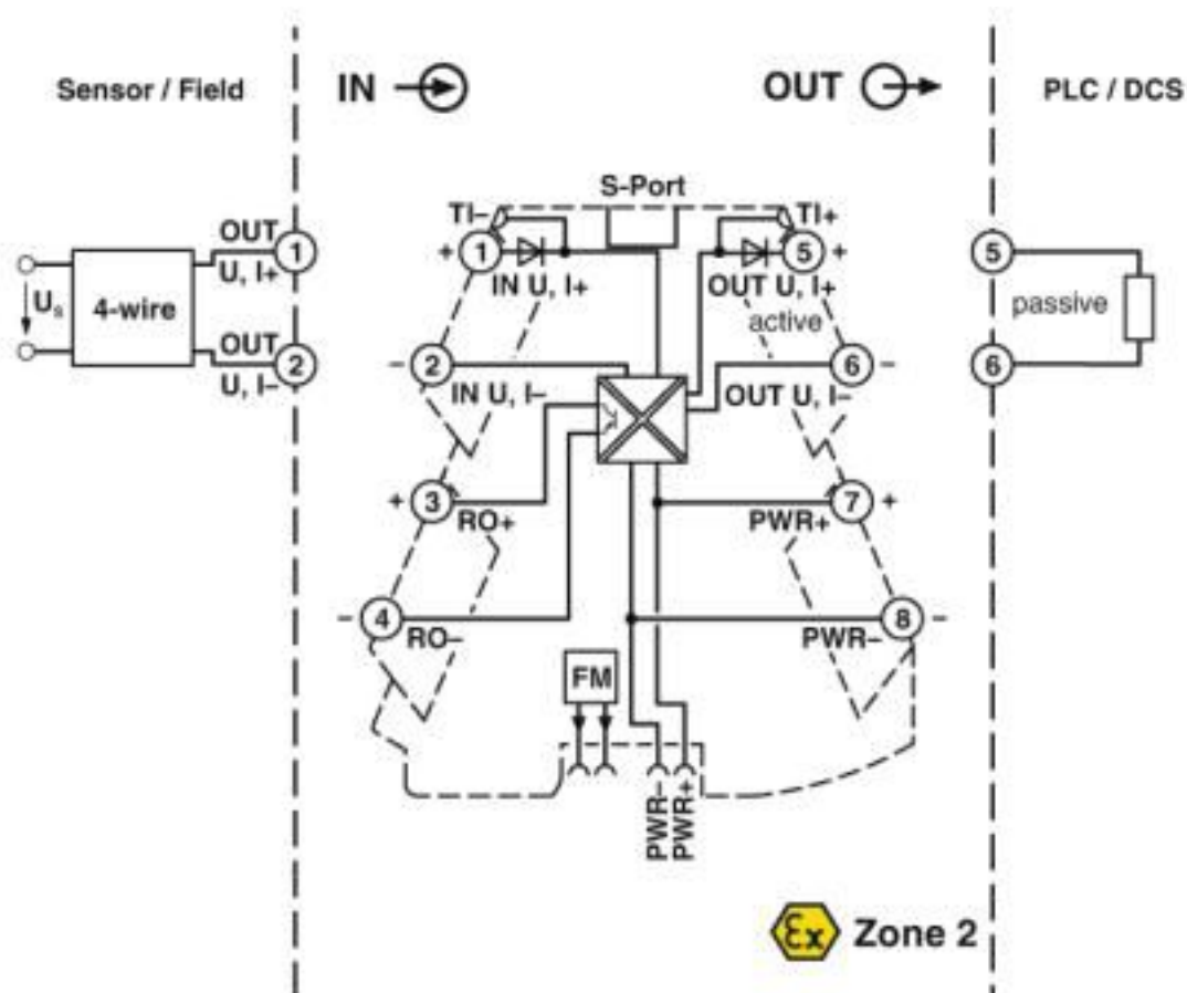
Block diagram
