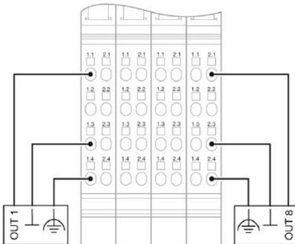
Connection diagram
