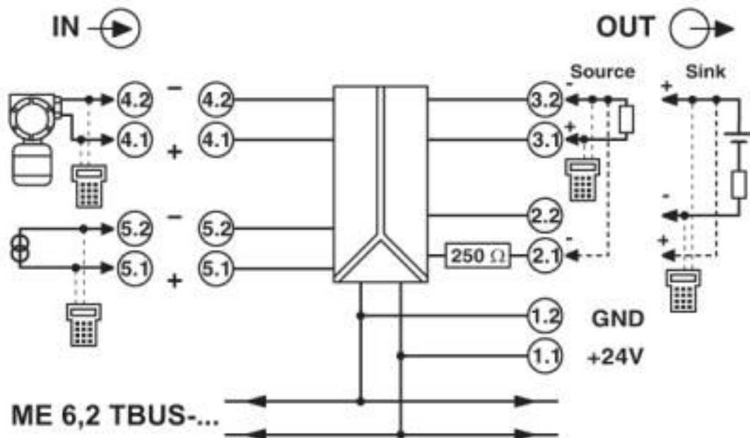
Block diagram
