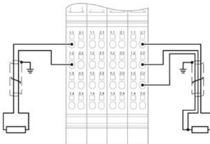
Connection diagram
