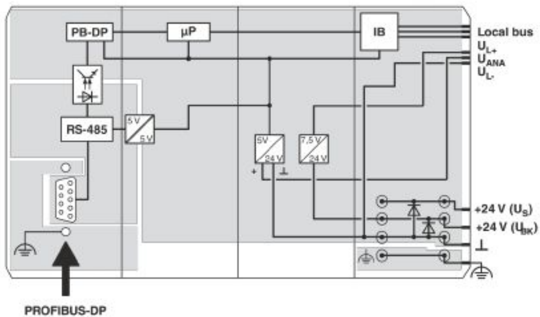
Block diagram
