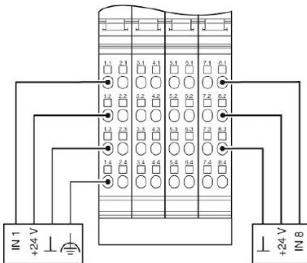
Connection diagram
