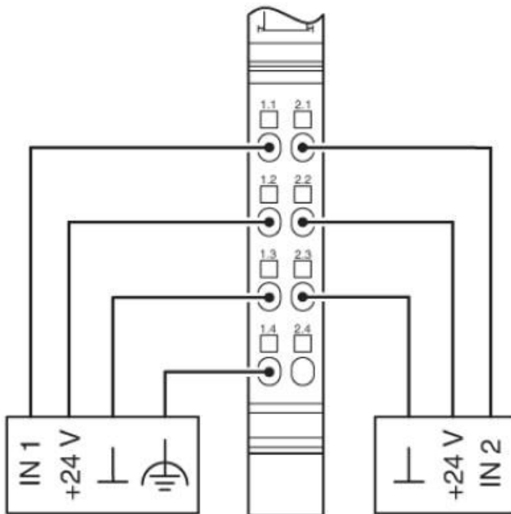
Connection diagram
