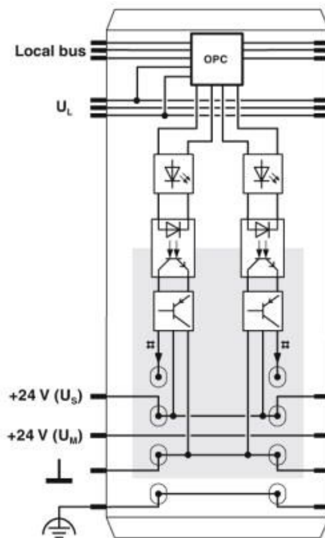
Block diagram
