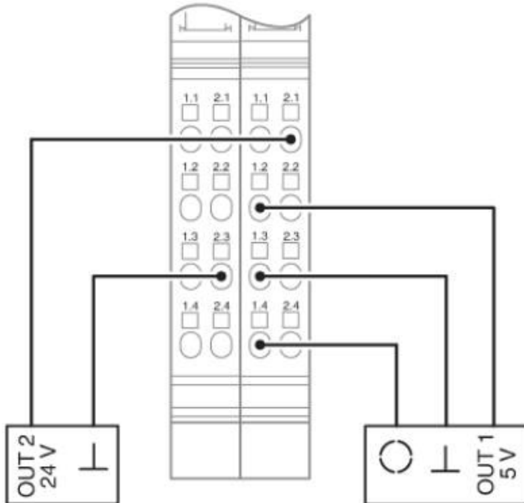
Connection diagram
