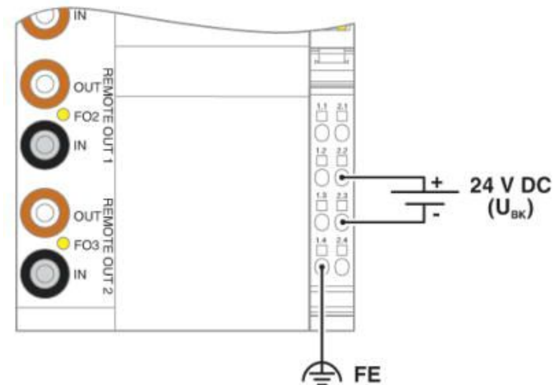
Connection diagram
