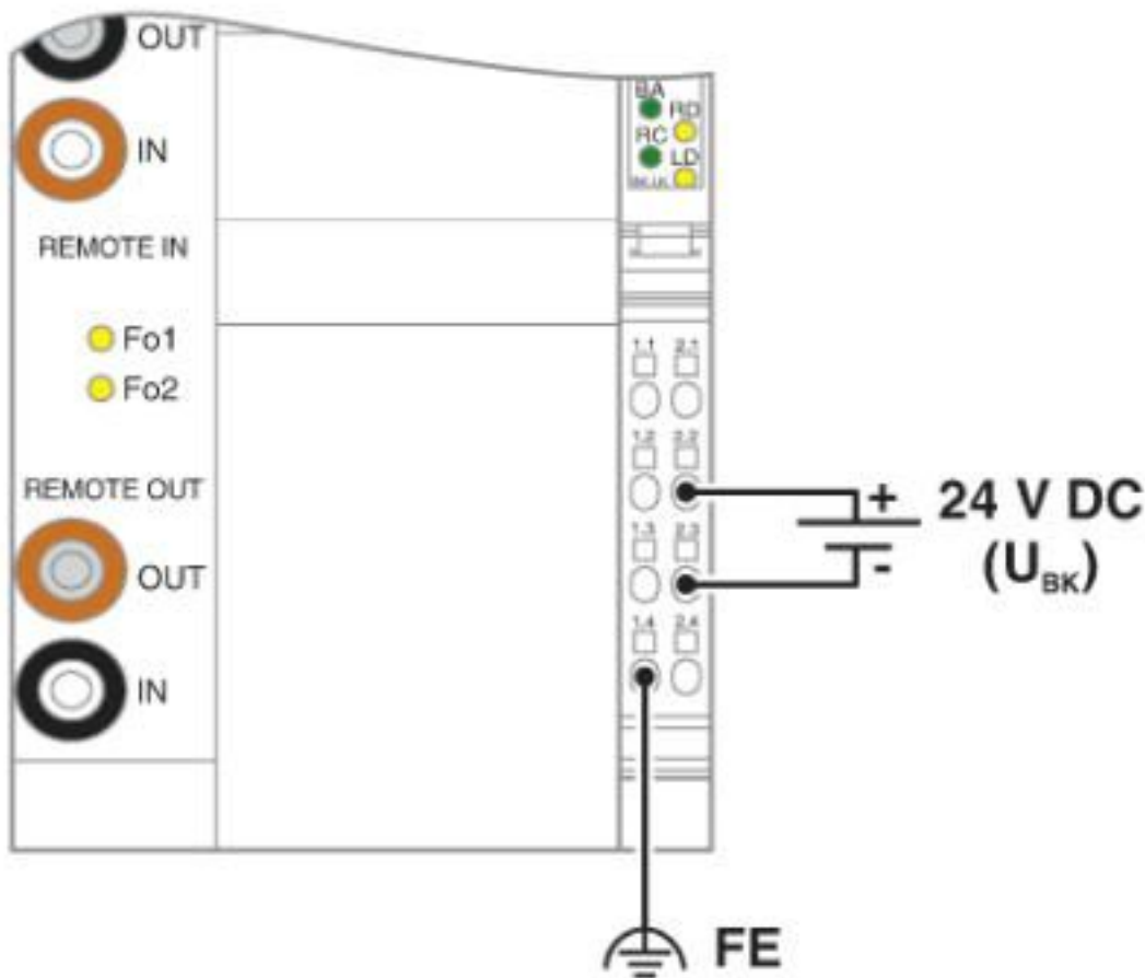
Connection diagram
