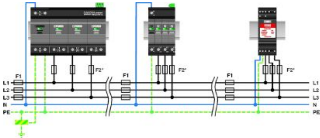
Application drawing
