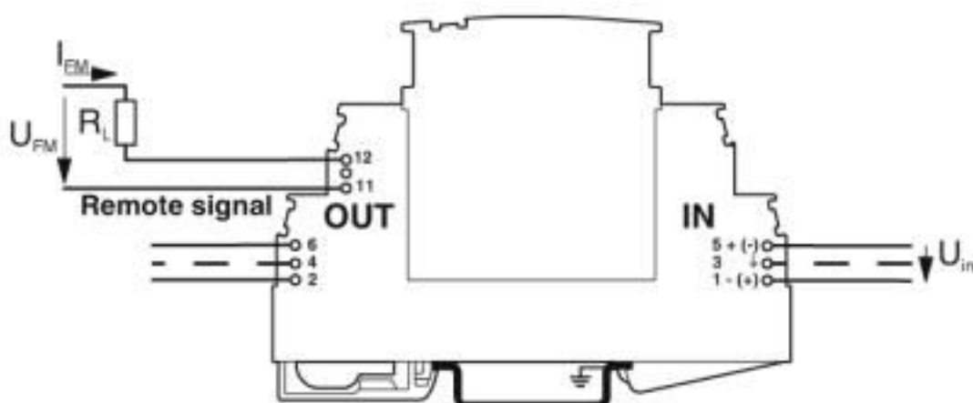
Connection diagram
