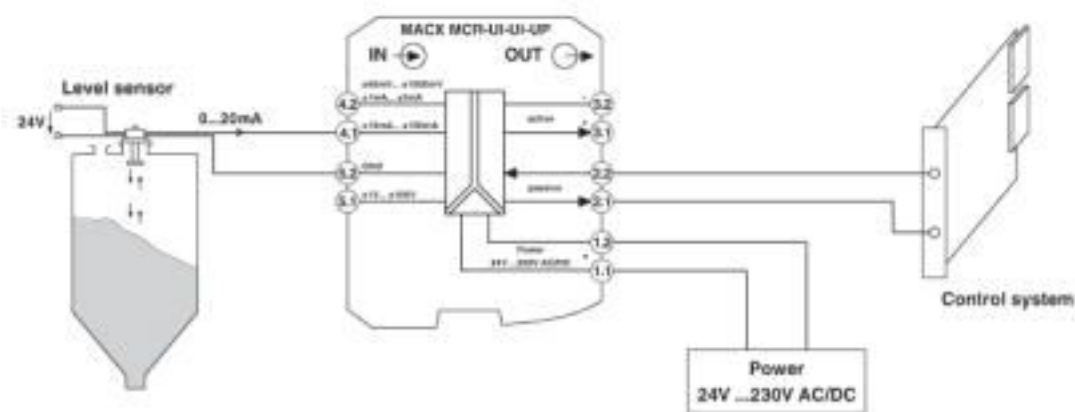
Application drawing
