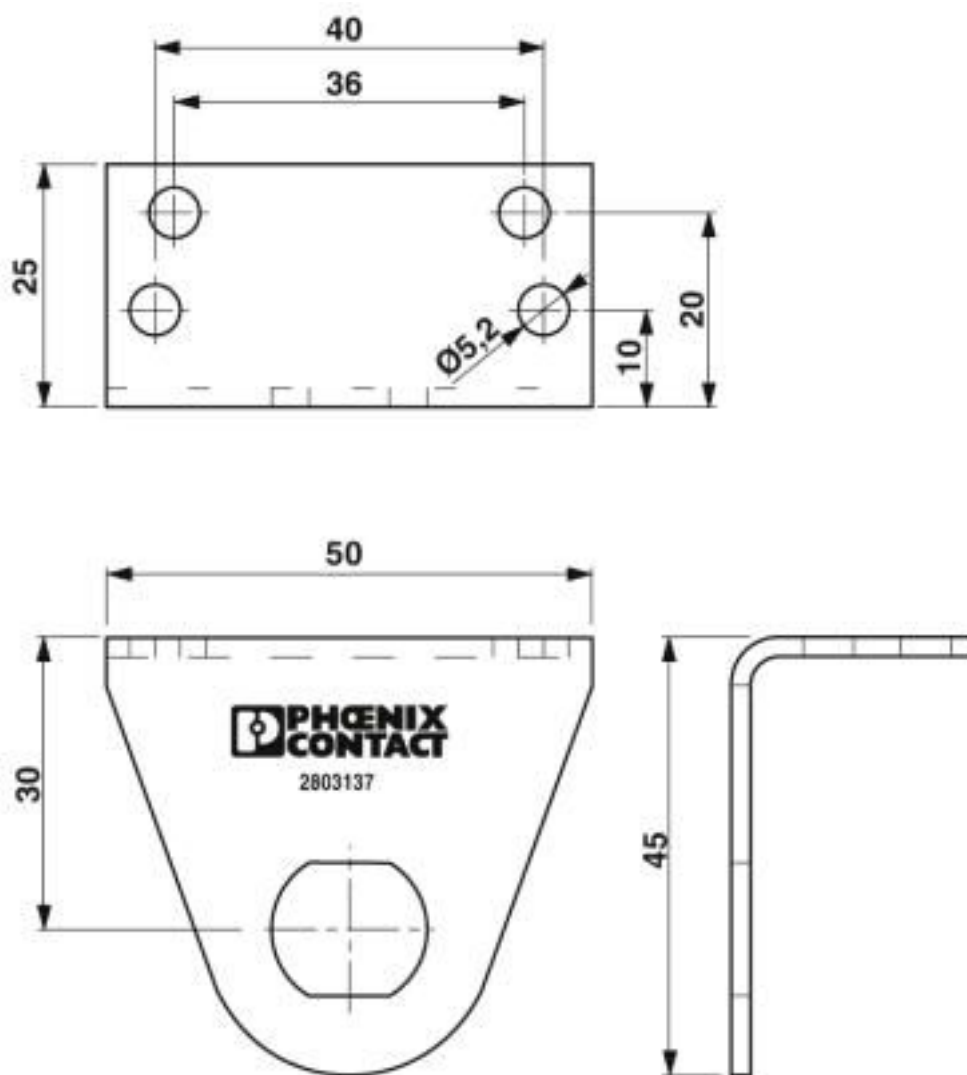
Dimensional drawing
