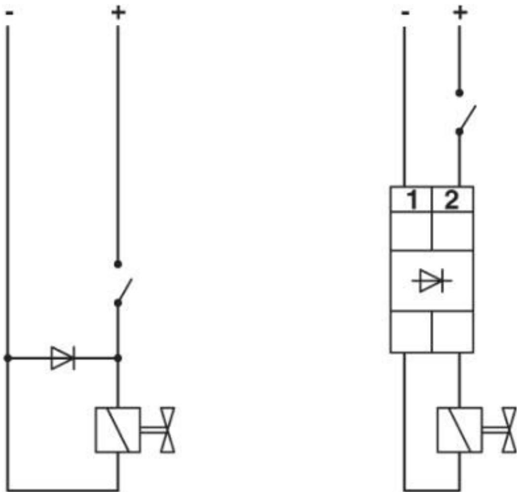
Circuit diagram
