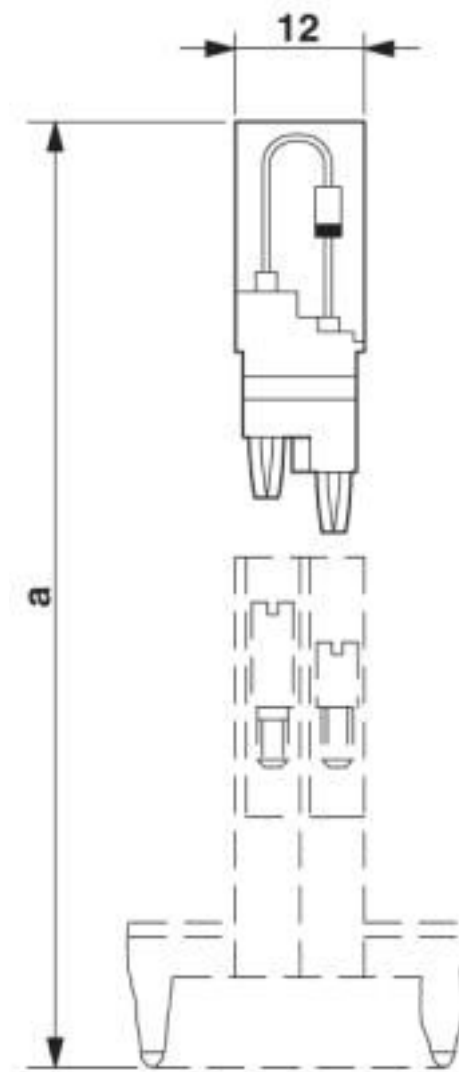
Dimensional drawing
