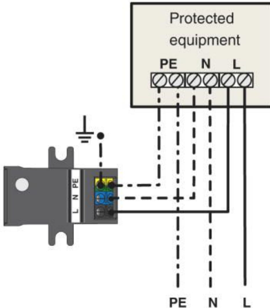
Application drawing
