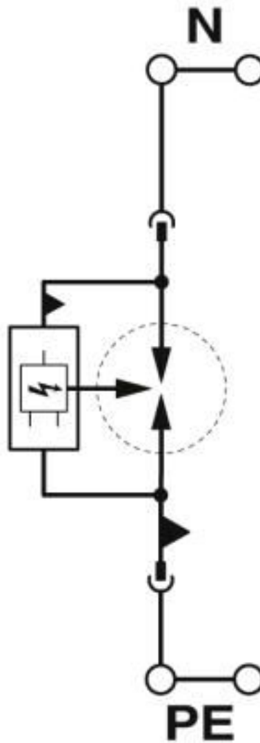
Circuit diagram
