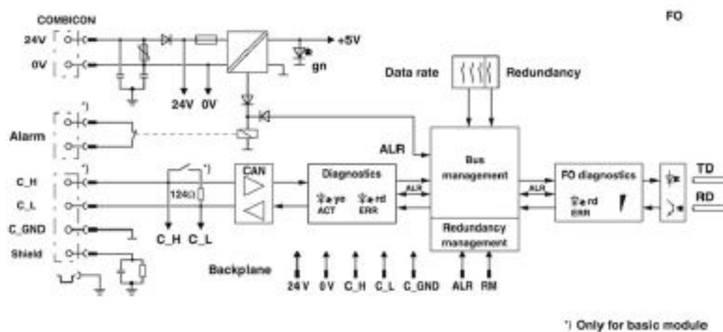
Block diagram
