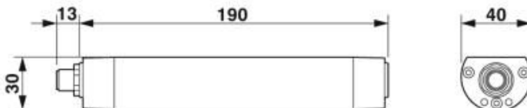
Dimensional drawing
