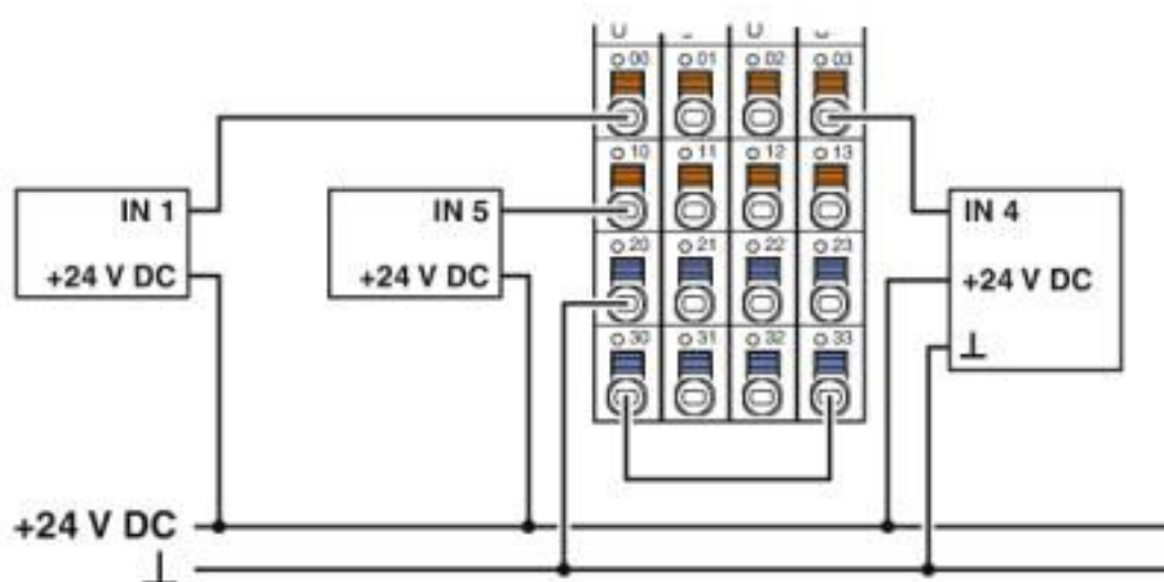
Connection diagram
