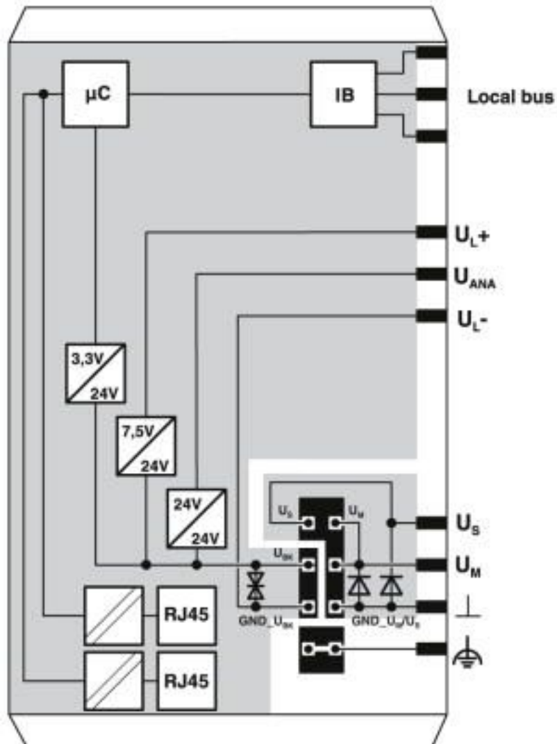
Block diagram
