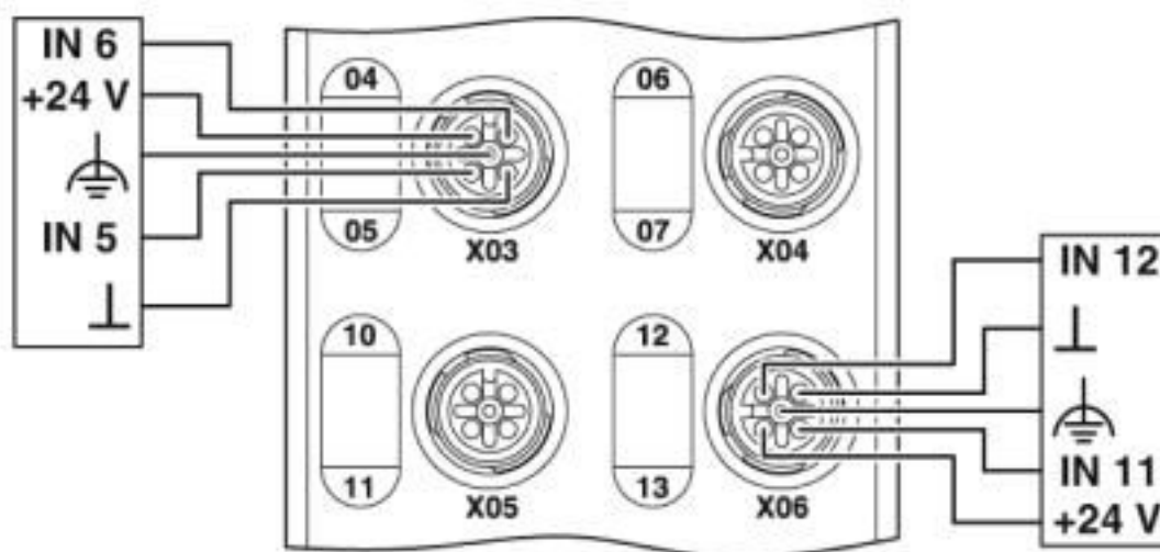
Connection diagram
