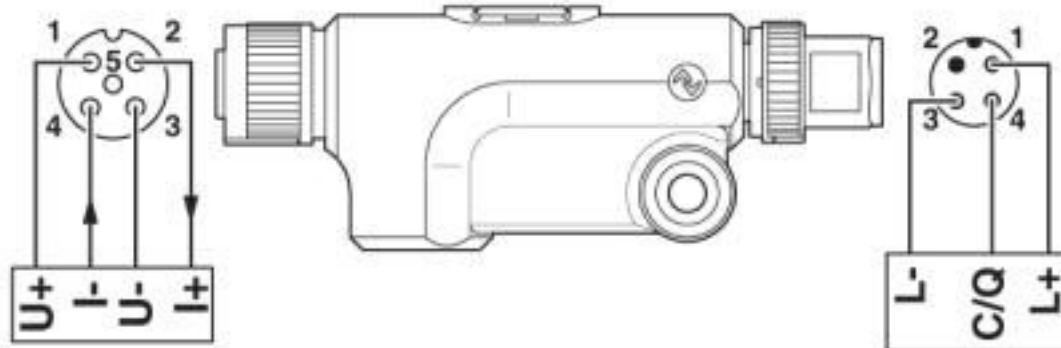
Block diagram
