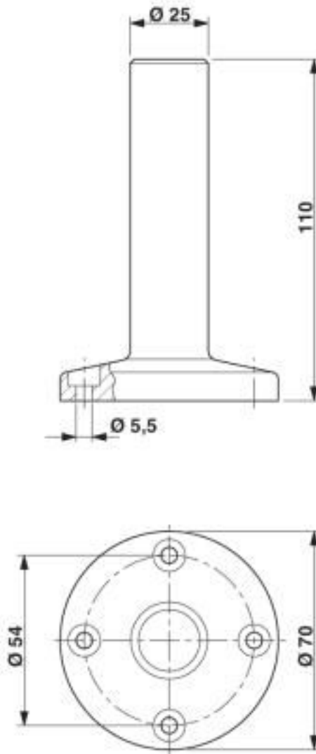
Dimensional drawing
