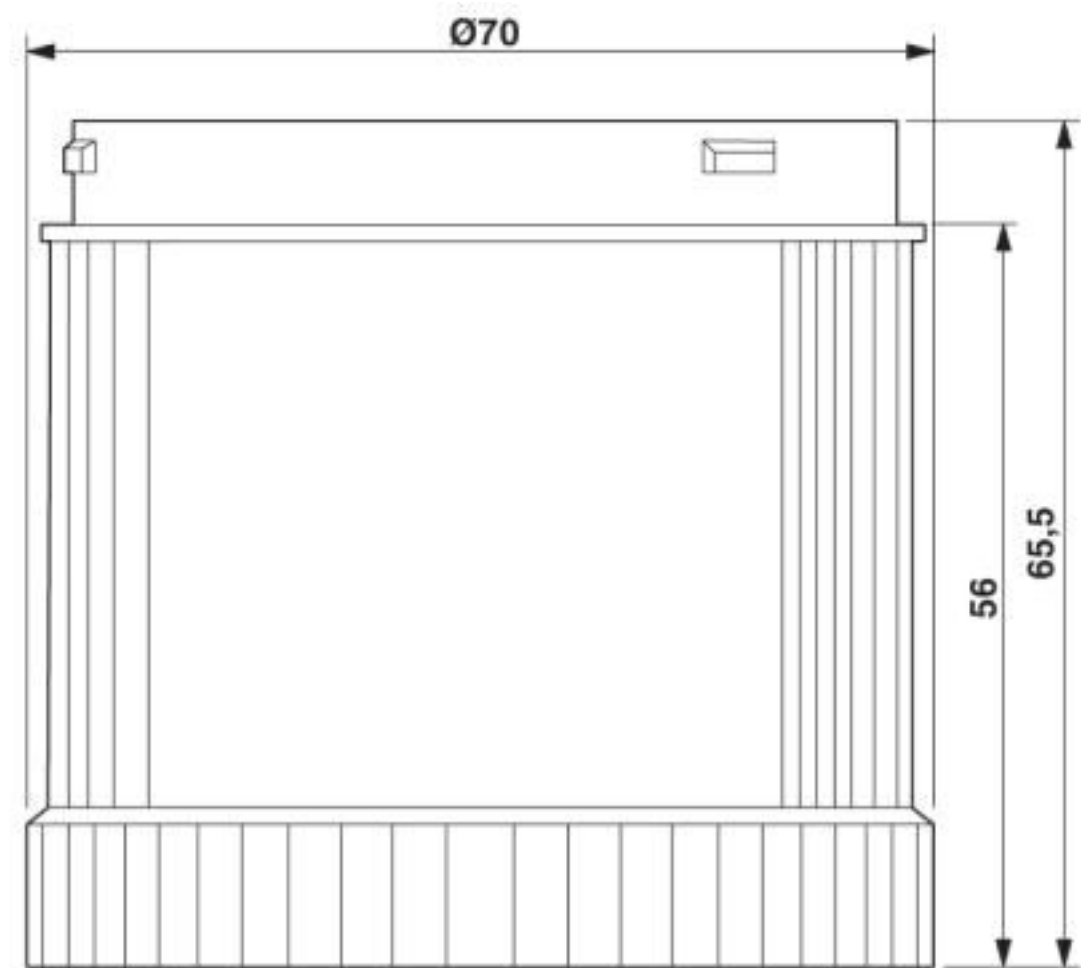
Dimensional drawing
