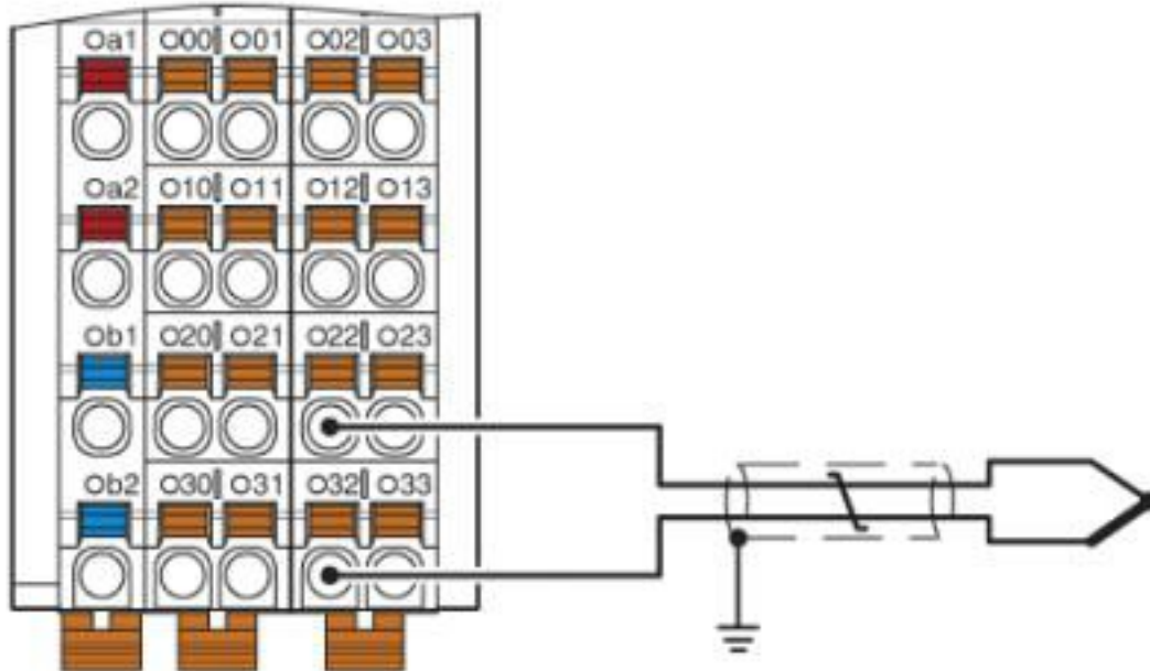
Connection diagram
