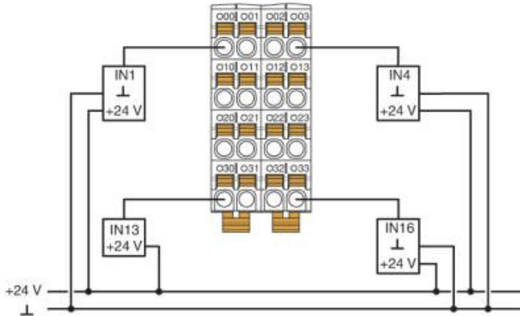
Connection diagram
