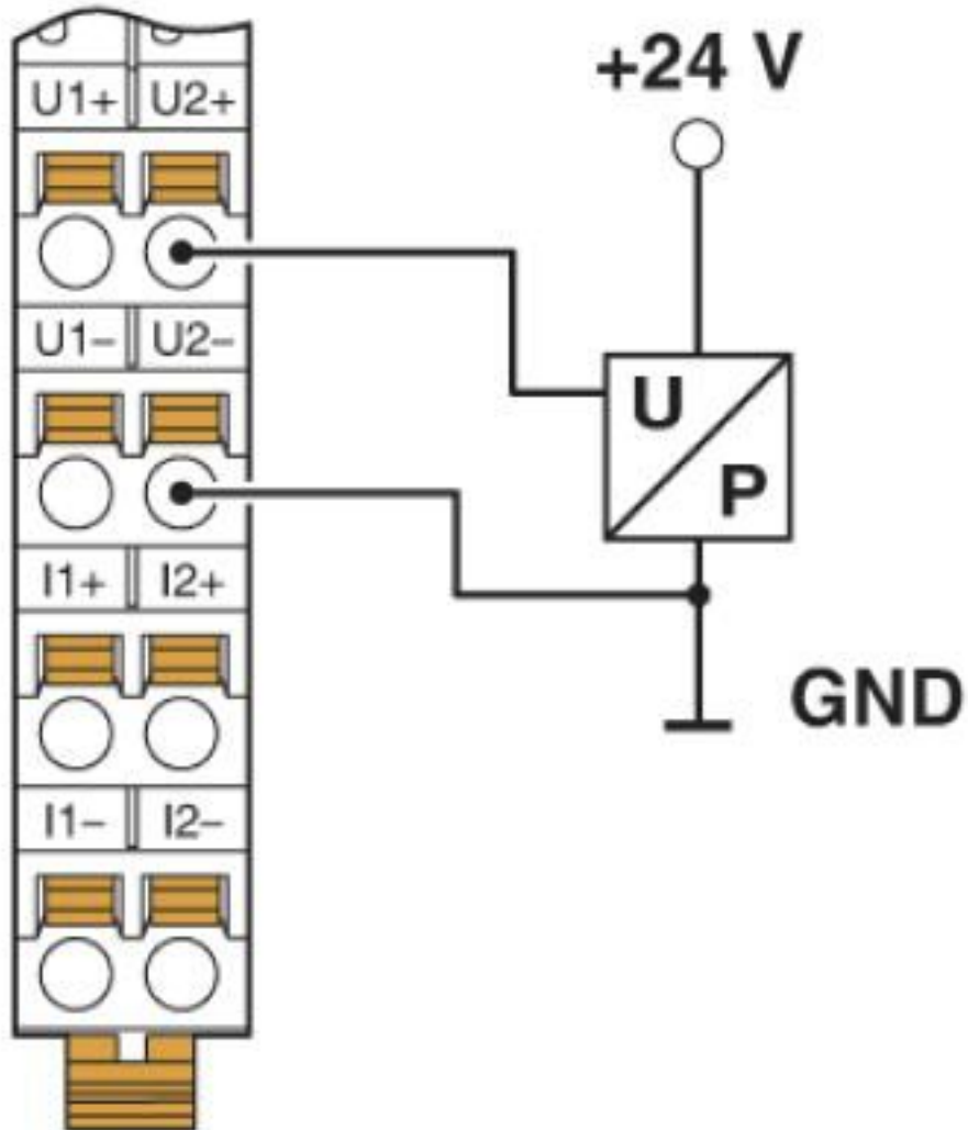
Connection diagram
