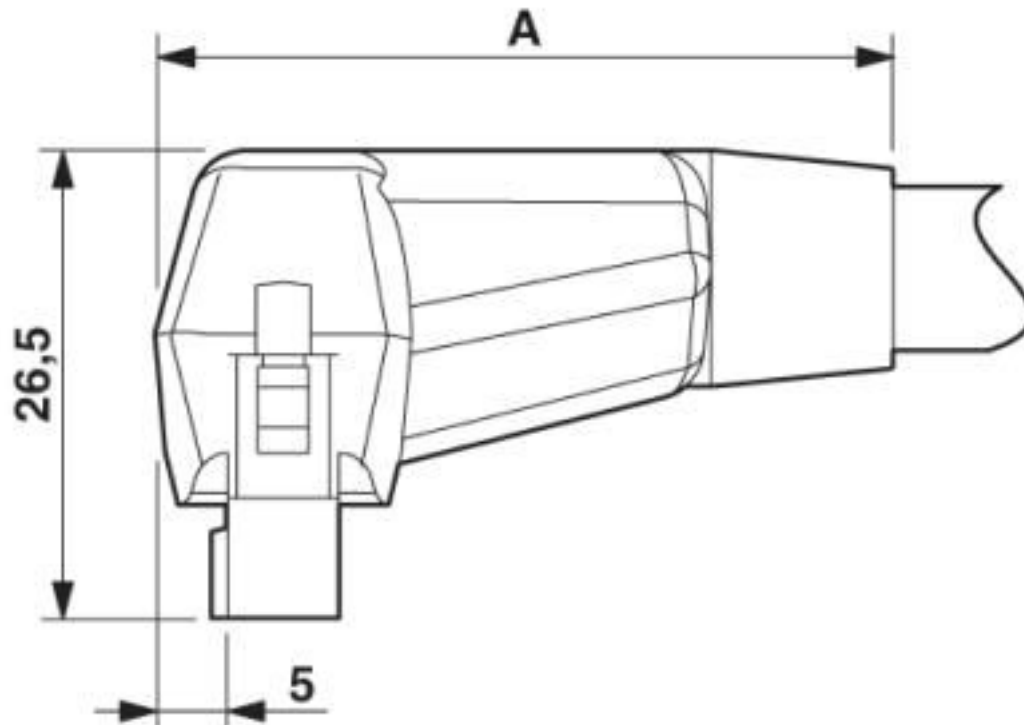
Dimensional drawing
