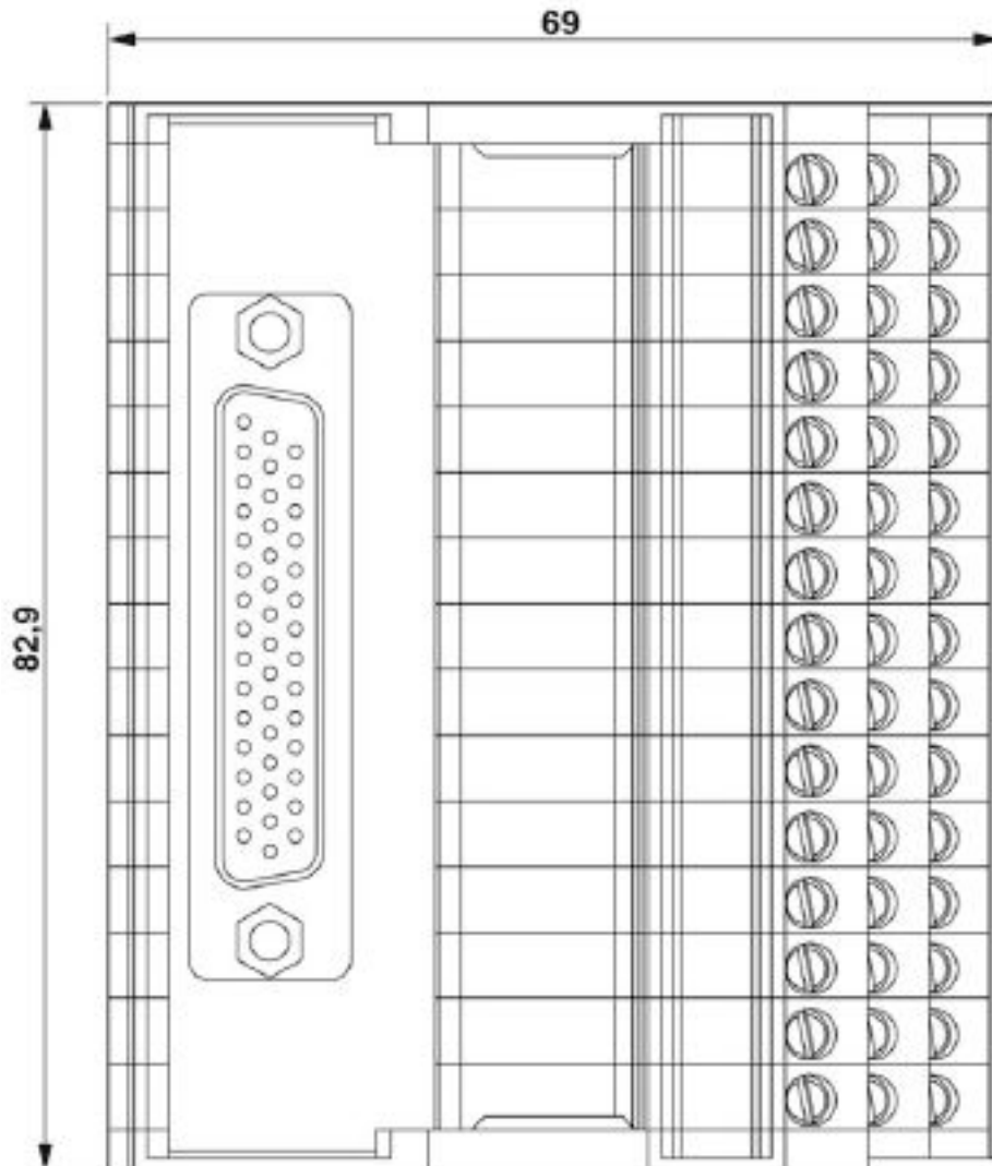
Dimensional drawing
