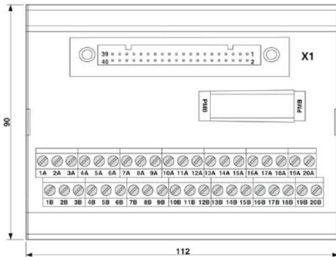
Dimensional drawing
