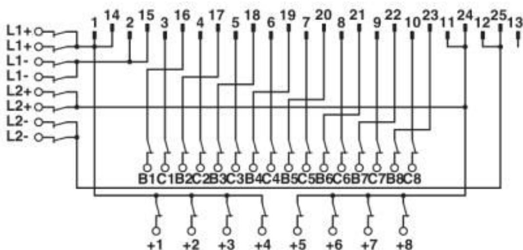
FLKM-D25 SUB/B/KDS3-MT/TU810/P connection scheme
